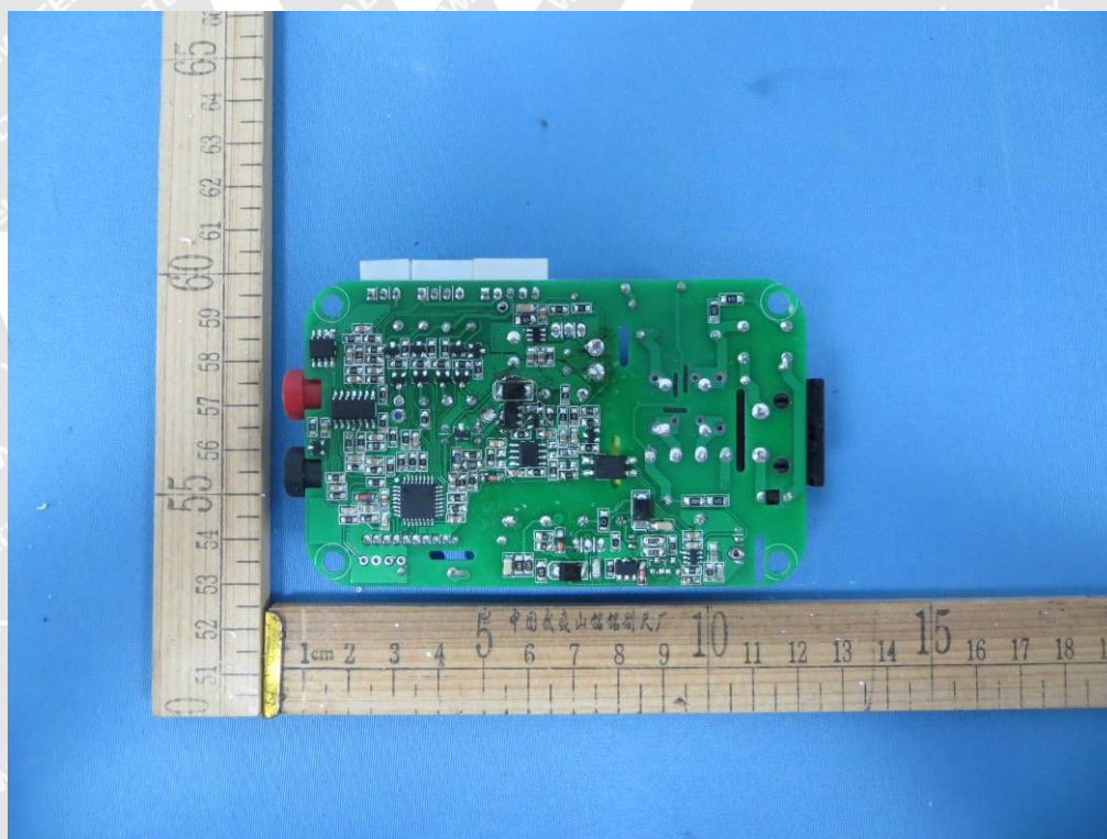
Photo 10 internal PCB bottom view
